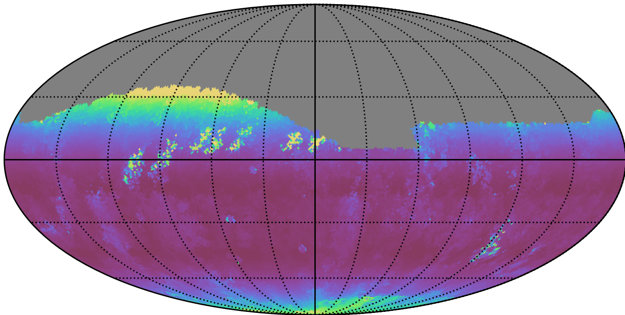
too_10_1v3.4_10yrs Yr 1 r band: Median airmass
