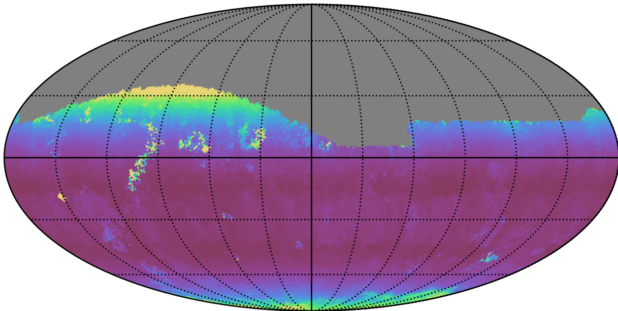
too_10_1v3.4_10yrs Yr 1 i band: Median airmass
