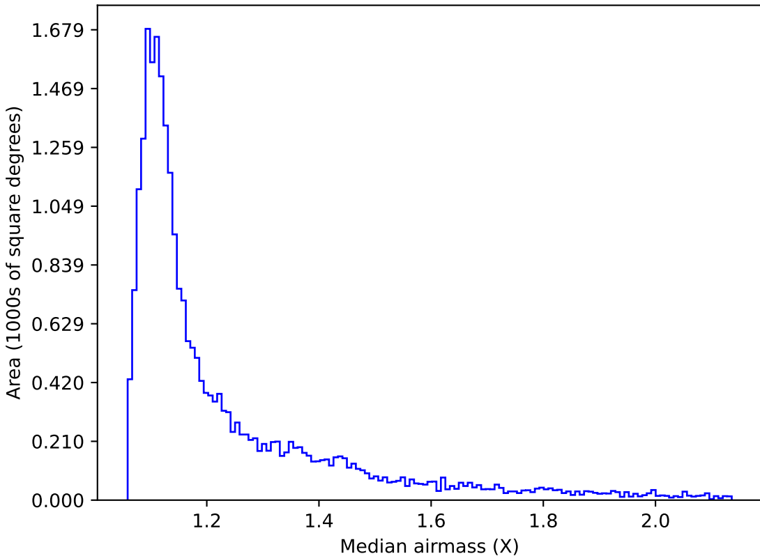
too_10_1v3.4_10yrs Yr 1 i band: Median airmass
