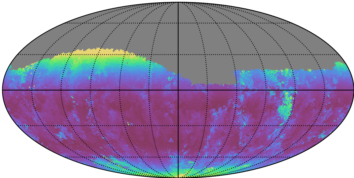
too_10_1v3.4_10yrs Yr 1 g band: Median airmass
