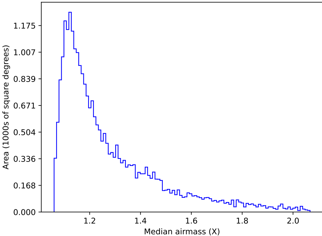
too_10_1v3.4_10yrs Yr 1 g band: Median airmass
