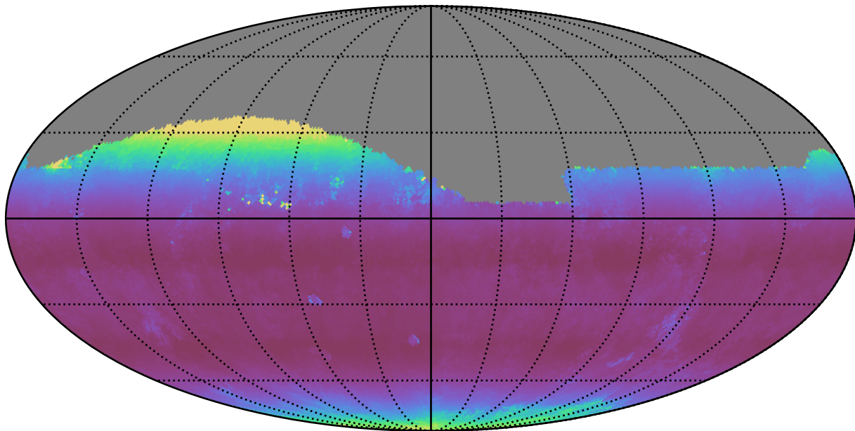
too_10_1v3.4_10yrs Yr 1 all bands: Median airmass
