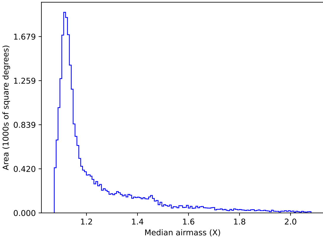
too_10_1v3.4_10yrs Yr 1 all bands: Median airmass
