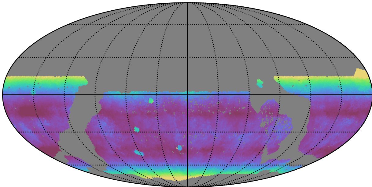
too_10_1v3.4_10yrs WFD z band: Median airmass
