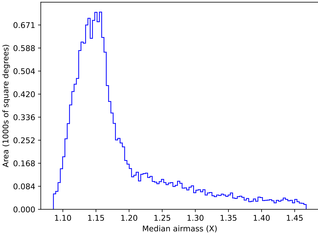
too_10_1v3.4_10yrs WFD z band: Median airmass
