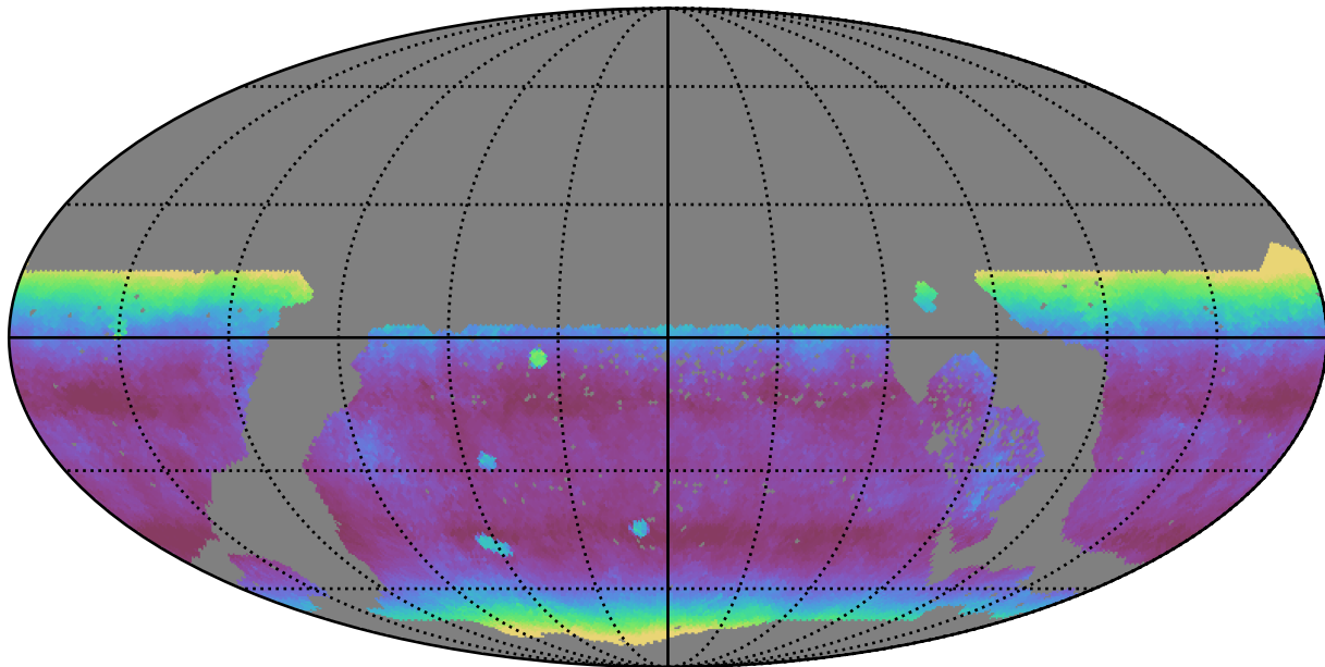
too_10_1v3.4_10yrs WFD y band: Median airmass
