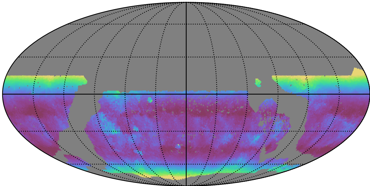
too_10_1v3.4_10yrs WFD u band: Median airmass
