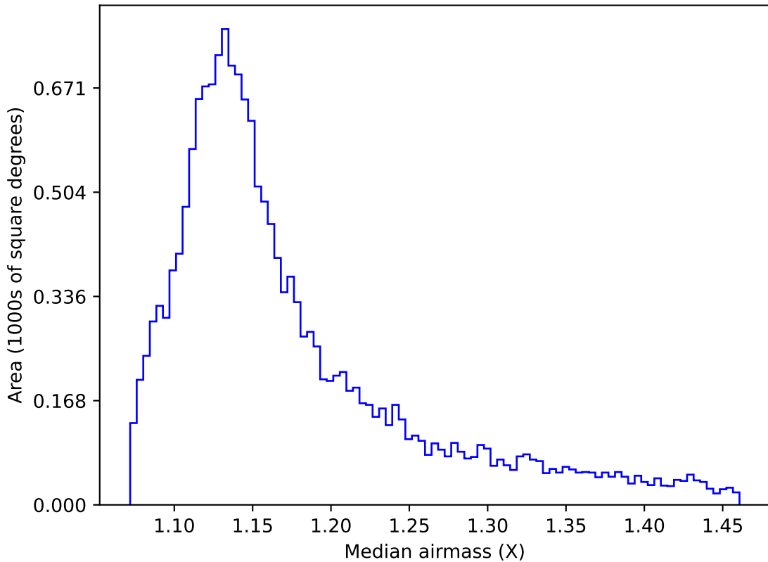
too_10_1v3.4_10yrs WFD u band: Median airmass
