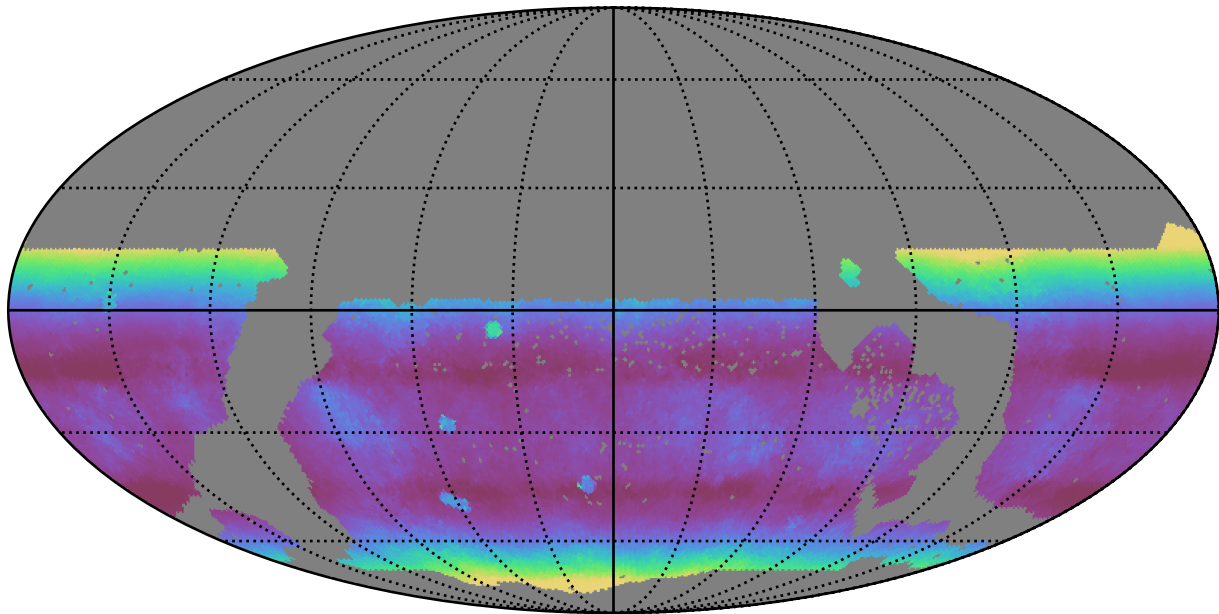
too_10_1v3.4_10yrs WFD r band: Median airmass
