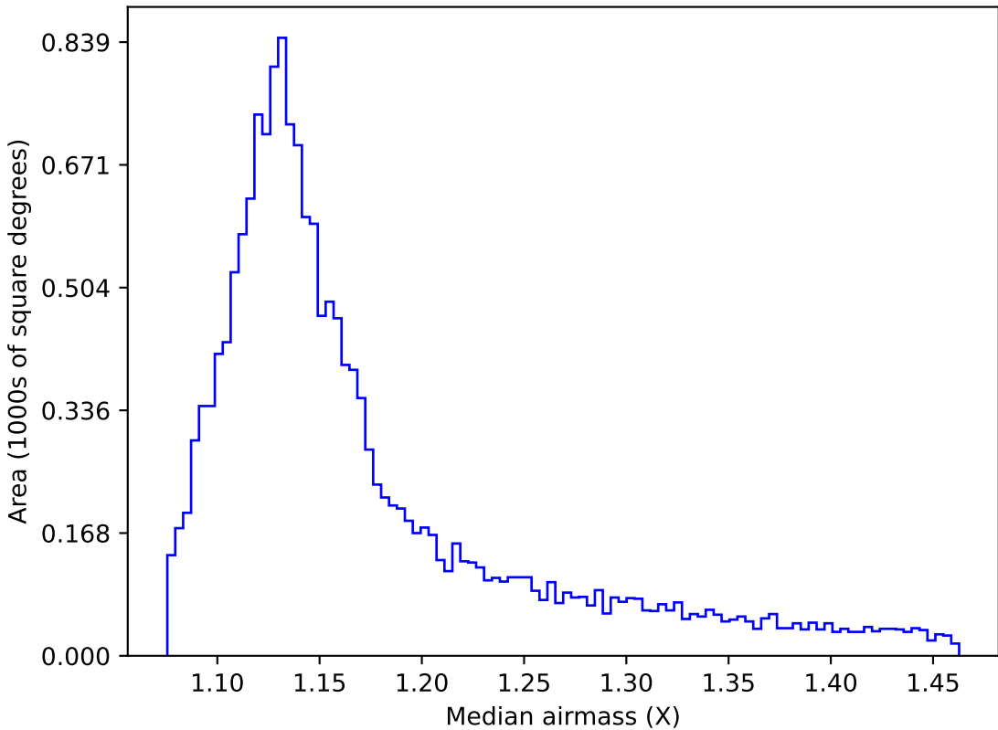
too_10_1v3.4_10yrs WFD r band: Median airmass
