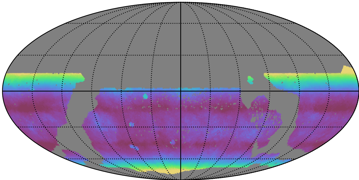
too_10_1v3.4_10yrs WFD i band: Median airmass
