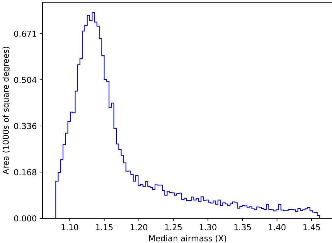
too_10_1v3.4_10yrs WFD i band: Median airmass
