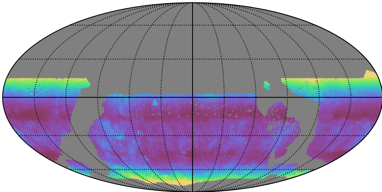
too_10_1v3.4_10yrs WFD g band: Median airmass
