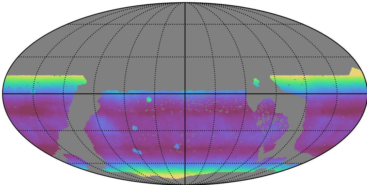
too_10_1v3.4_10yrs WFD all bands: Median airmass
