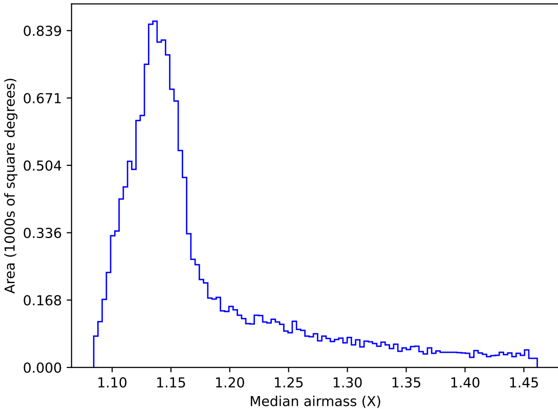
too_10_1v3.4_10yrs WFD all bands: Median airmass
