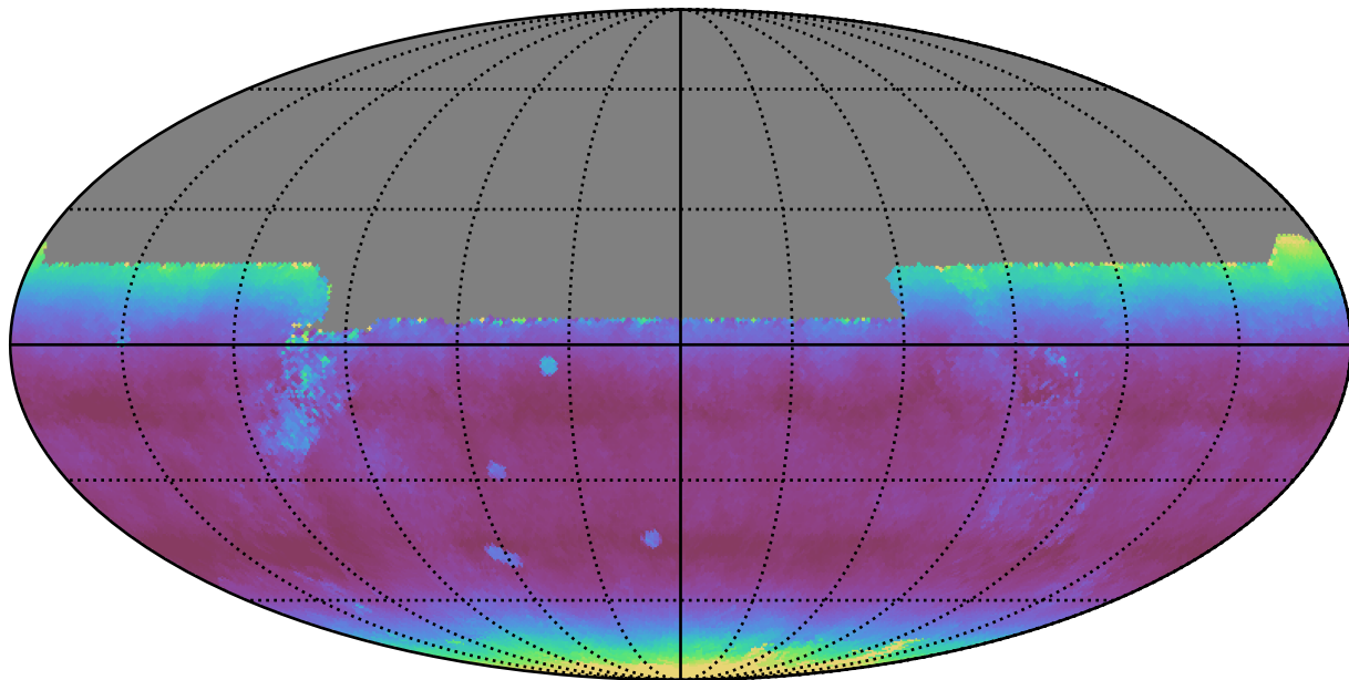
too_10_1v3.4_10yrs All sky y band: Median airmass
