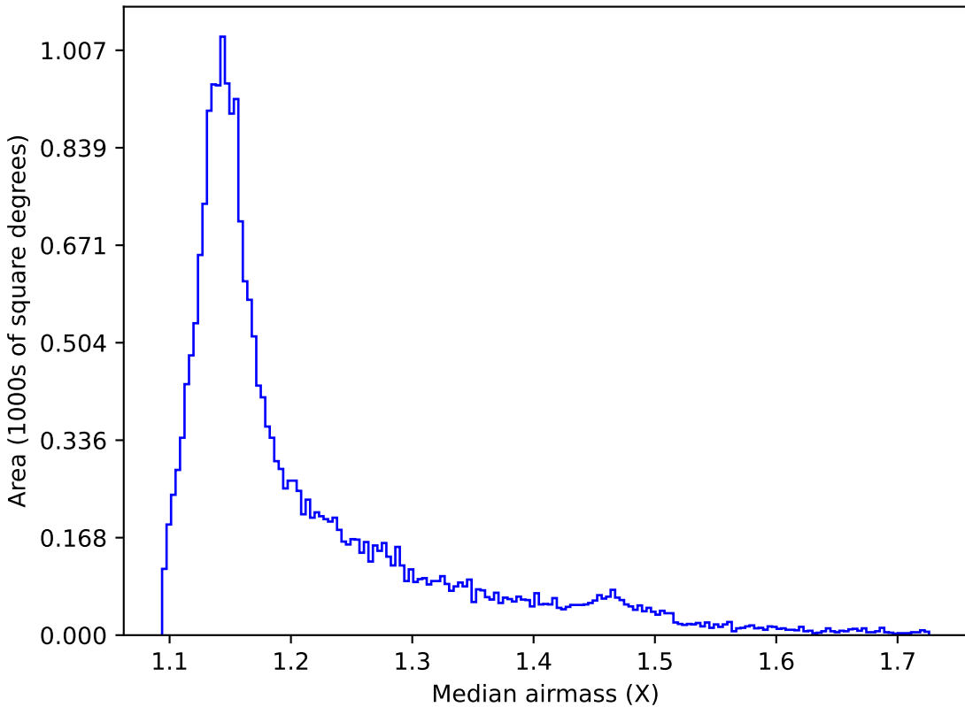
too_10_1v3.4_10yrs All sky y band: Median airmass
