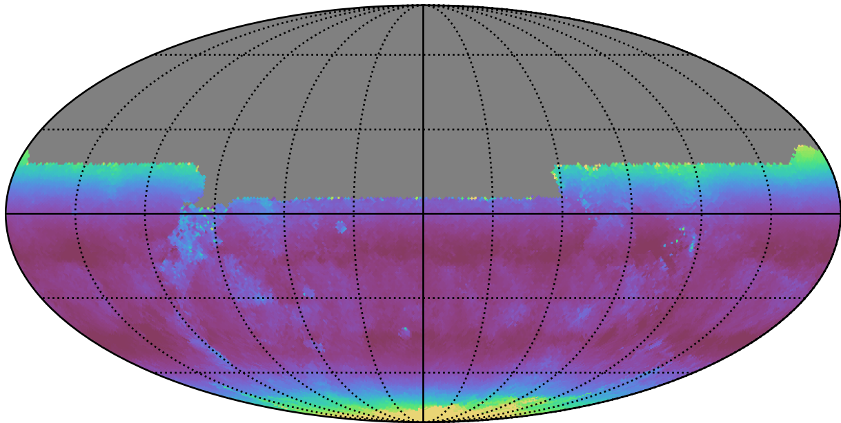
too_10_1v3.4_10yrs All sky u band: Median airmass
