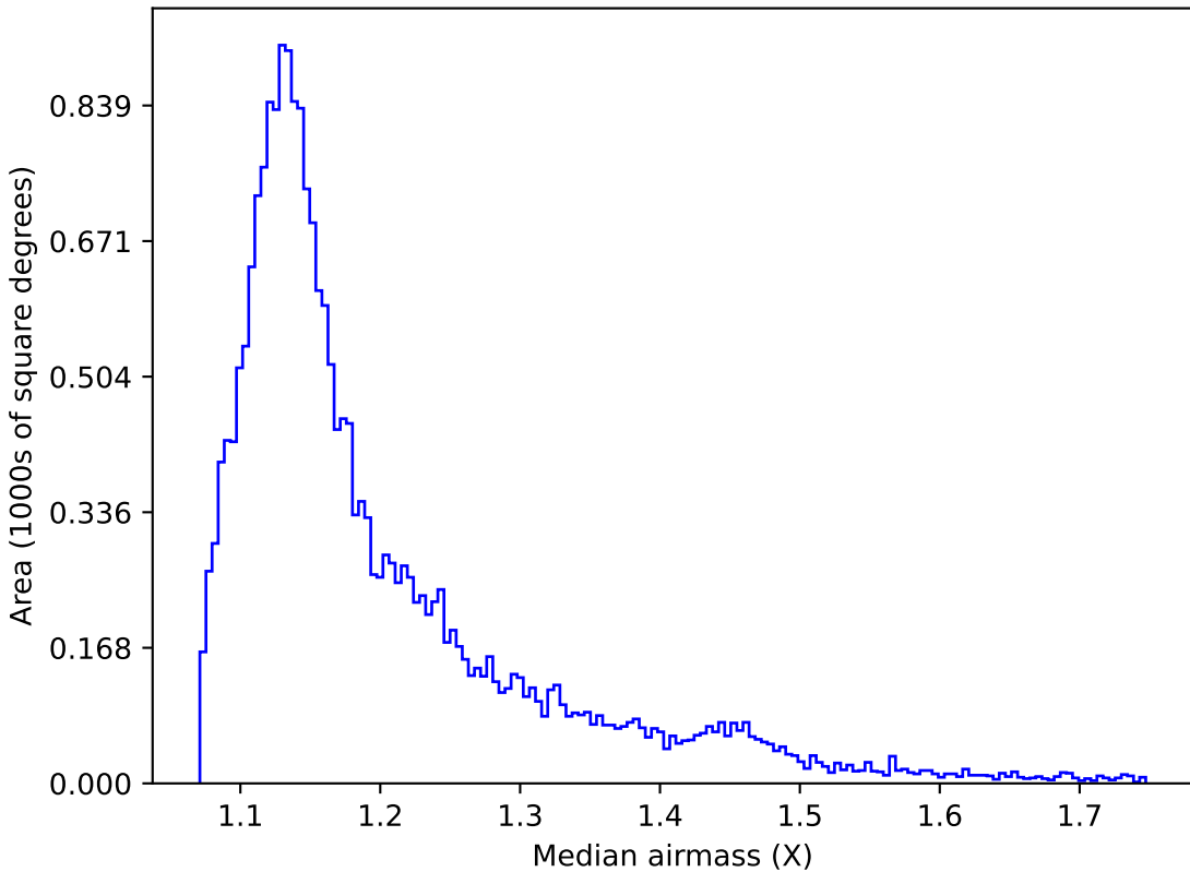
too_10_1v3.4_10yrs All sky u band: Median airmass
