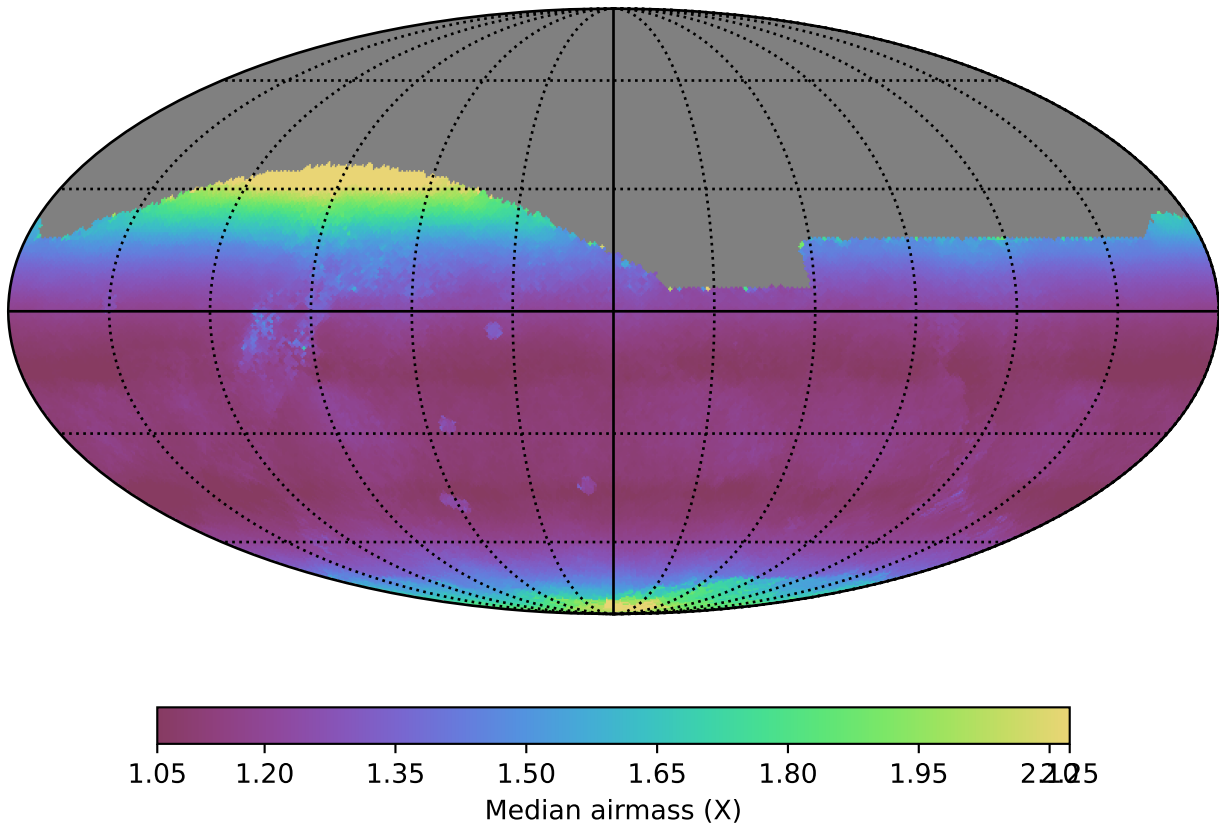
too_10_1v3.4_10yrs All sky r band: Median airmass
