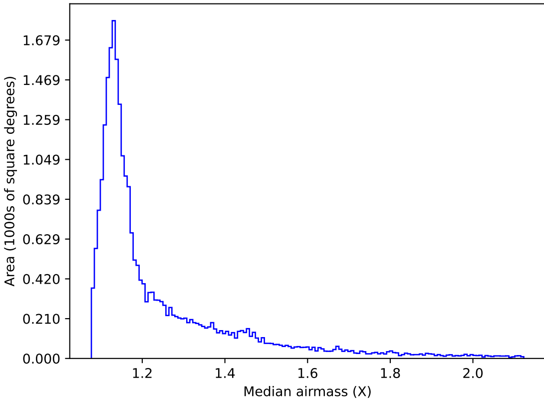
too_10_1v3.4_10yrs All sky r band: Median airmass
