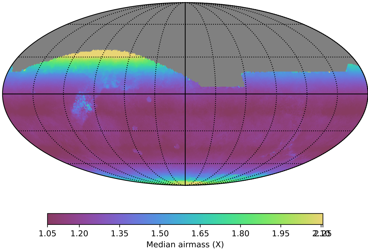
too_10_1v3.4_10yrs All sky i band: Median airmass
