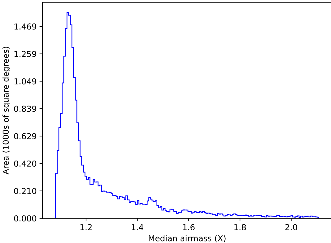
too_10_1v3.4_10yrs All sky i band: Median airmass
