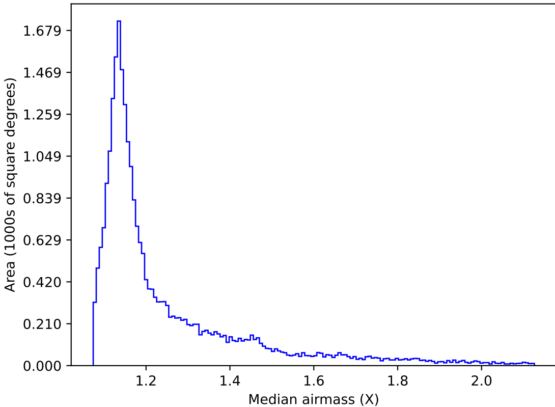
too_10_1v3.4_10yrs All sky g band: Median airmass
