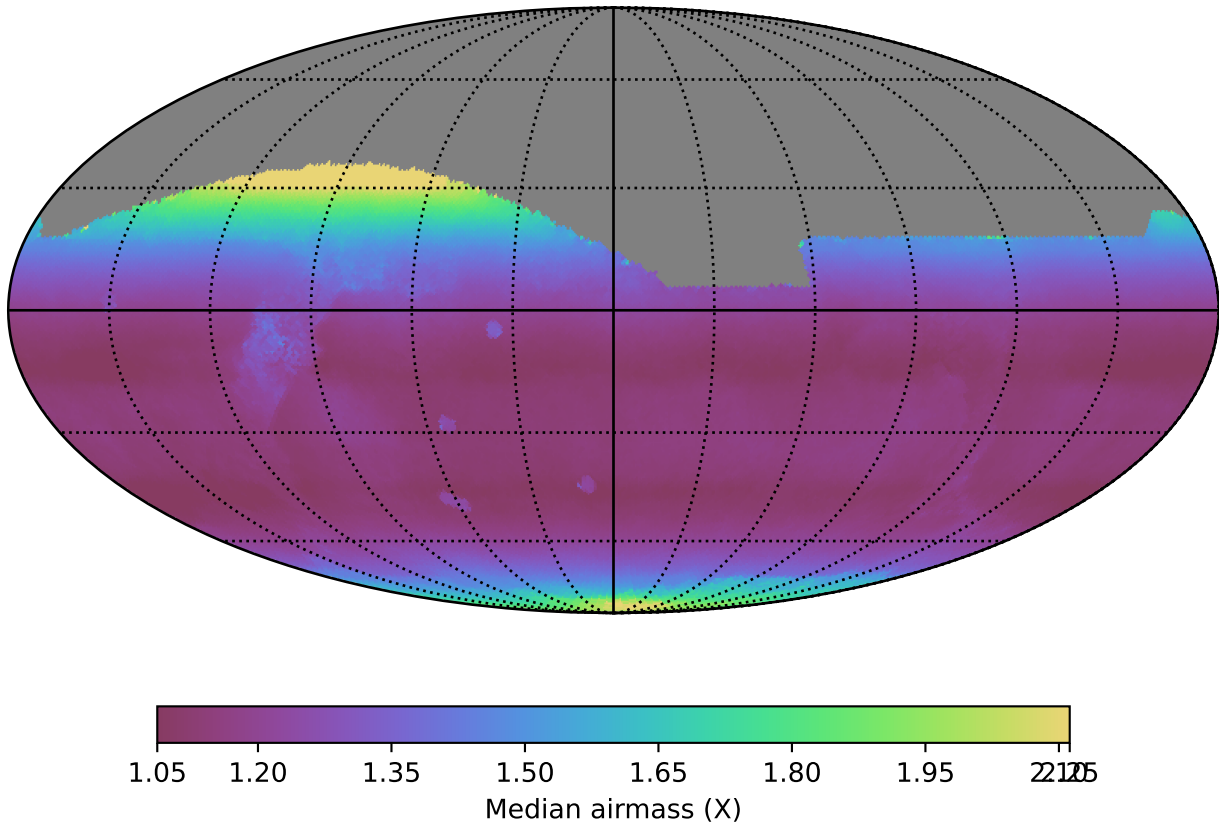
too_10_1v3.4_10yrs All sky all bands: Median airmass
