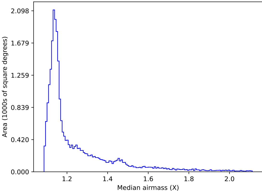
too_10_1v3.4_10yrs All sky all bands: Median airmass
