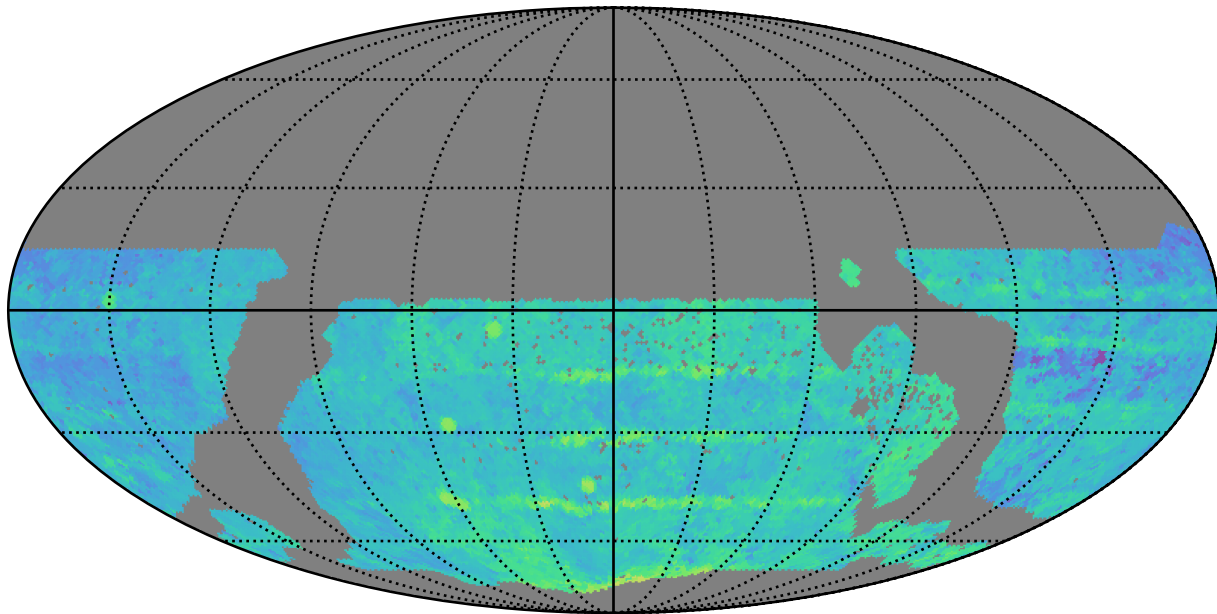
too_10_1v3.4_10yrs WFD z band: Median Season Length
