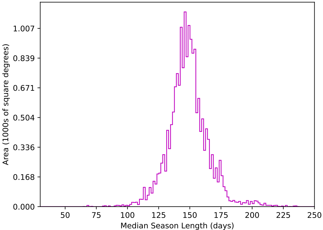
too_10_1v3.4_10yrs WFD z band: Median Season Length
