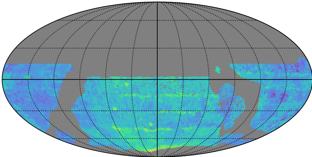
too_10_1v3.4_10yrs WFD y band: Median Season Length
