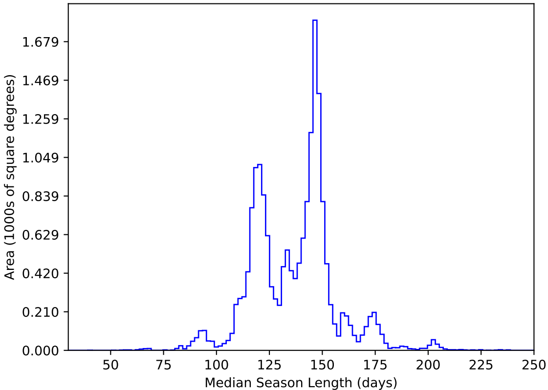
too_10_1v3.4_10yrs WFD y band: Median Season Length
