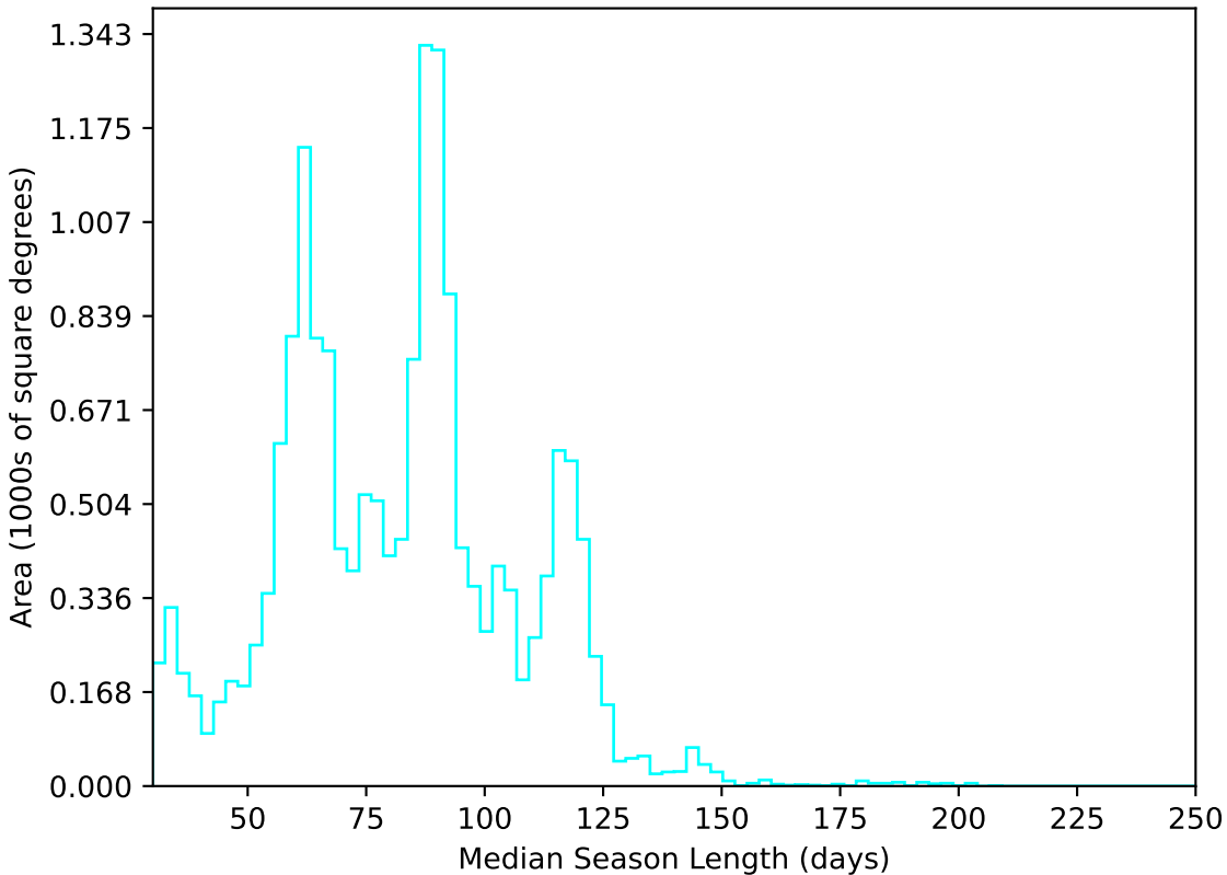
too_10_1v3.4_10yrs WFD u band: Median Season Length
