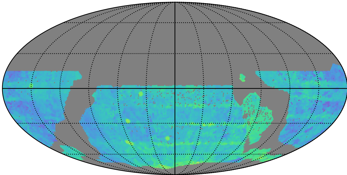
too_10_1v3.4_10yrs WFD r band: Median Season Length
