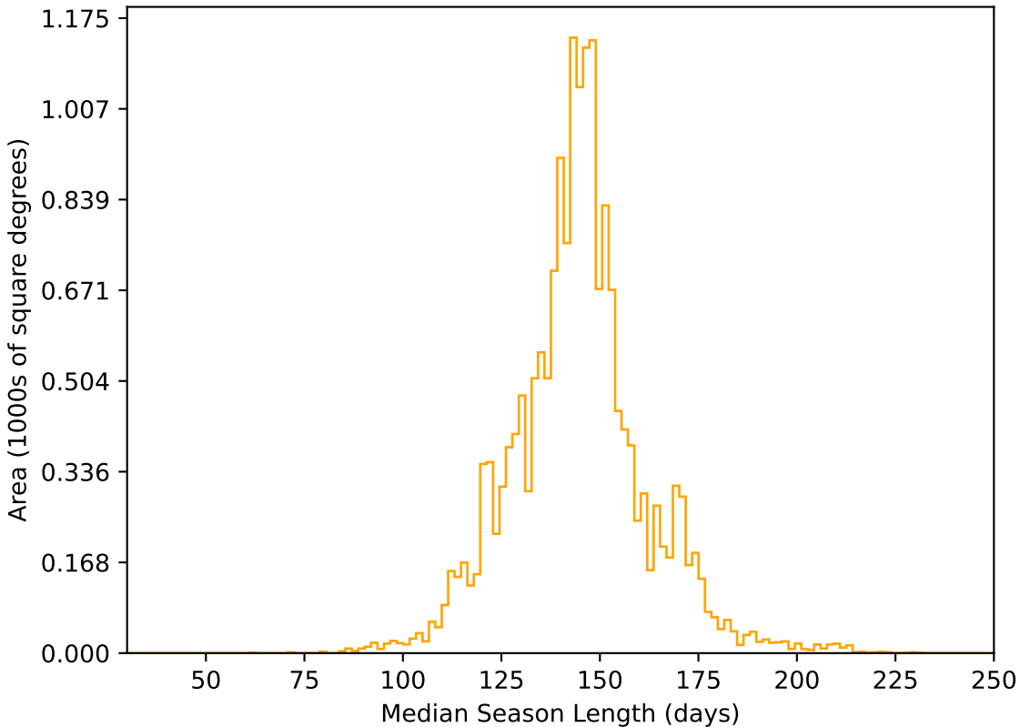
too_10_1v3.4_10yrs WFD r band: Median Season Length
