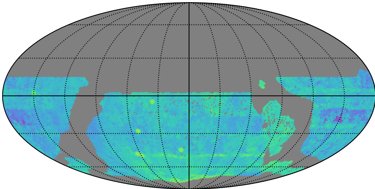
too_10_1v3.4_10yrs WFD i band: Median Season Length
