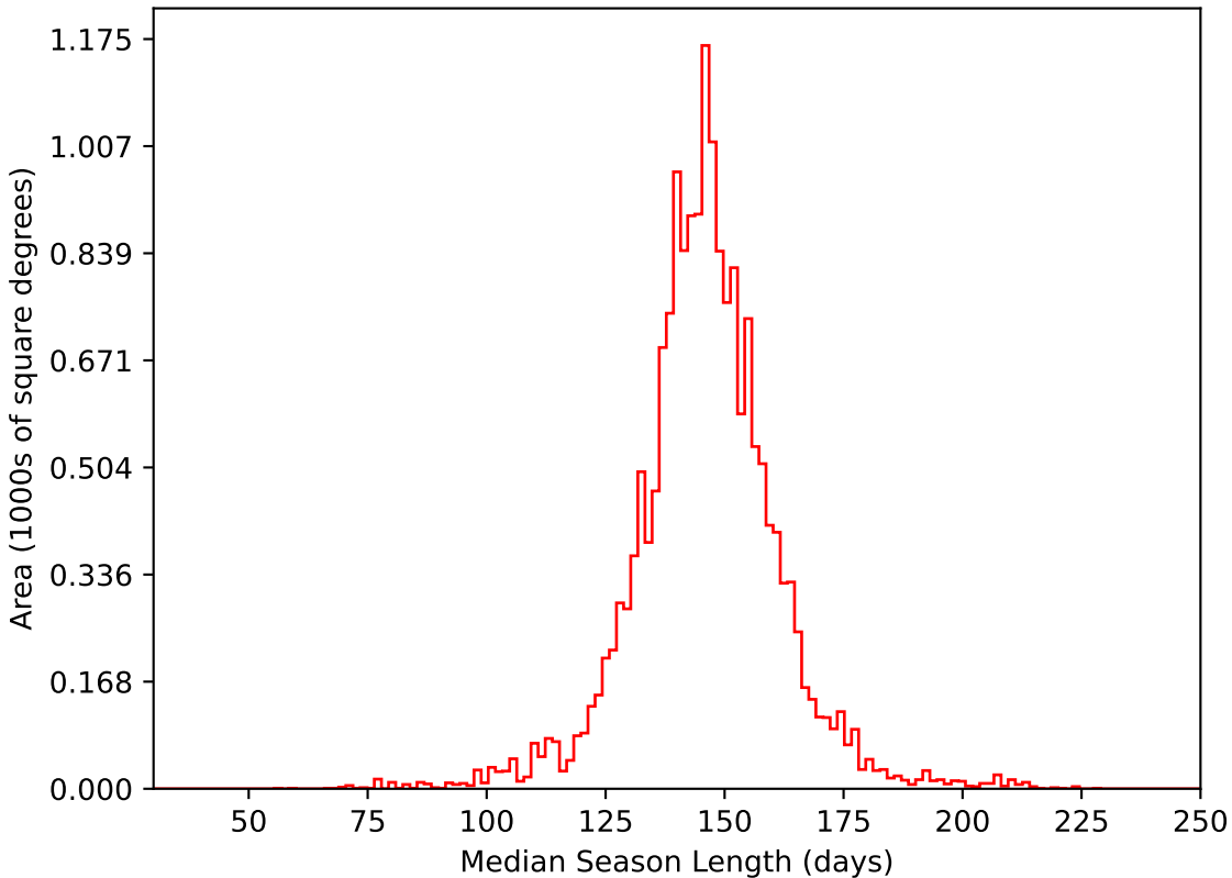
too_10_1v3.4_10yrs WFD i band: Median Season Length
