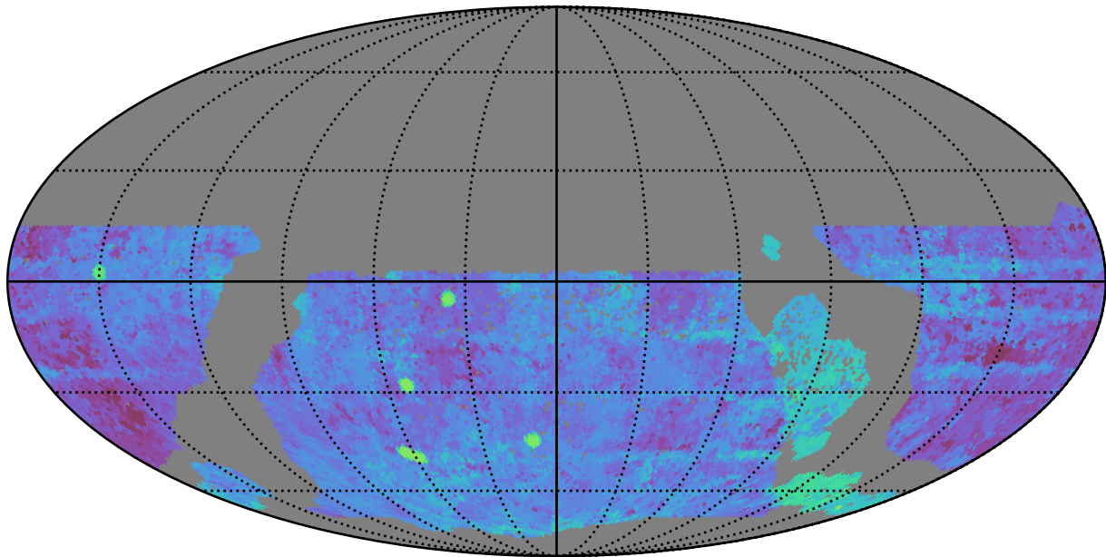
too_10_1v3.4_10yrs WFD g band: Median Season Length
