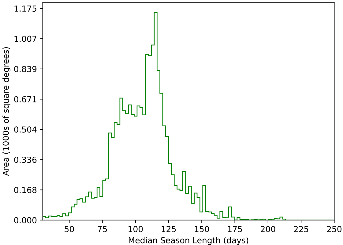
too_10_1v3.4_10yrs WFD g band: Median Season Length
