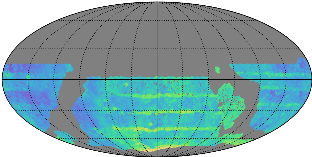
too_10_1v3.4_10yrs WFD all bands: Median Season Length
