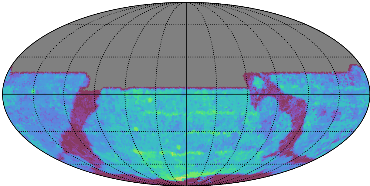
too_10_1v3.4_10yrs All sky y band: Median Season Length
