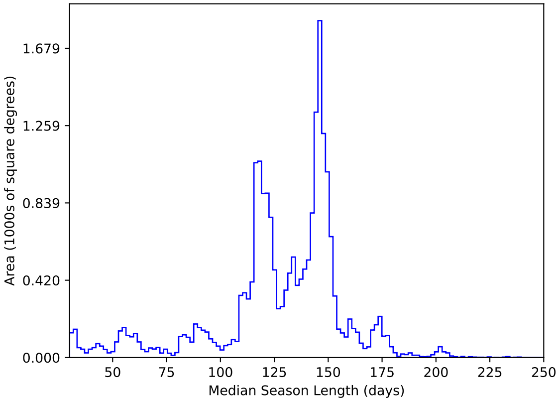
too_10_1v3.4_10yrs All sky y band: Median Season Length
