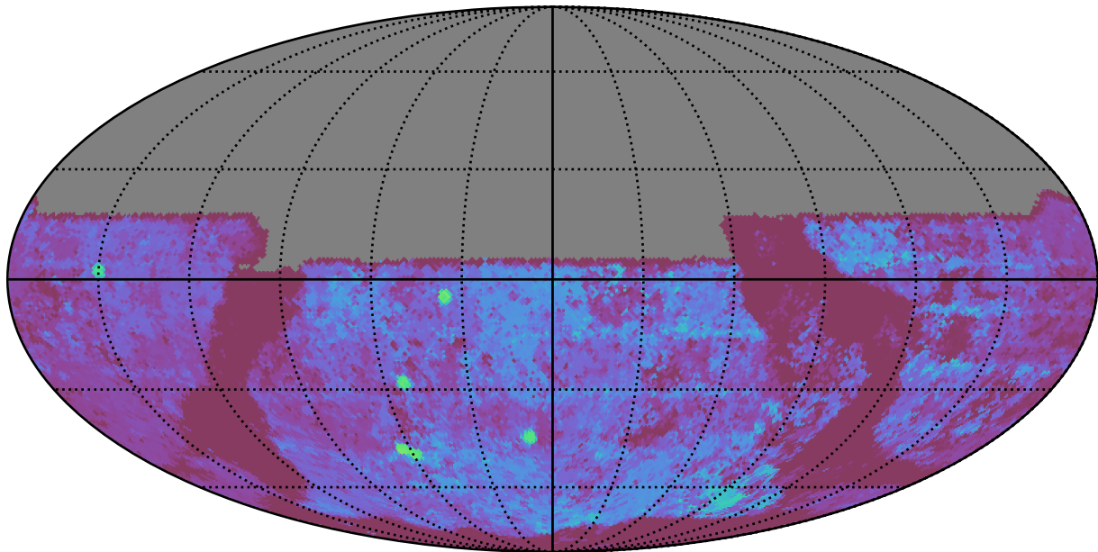
too_10_1v3.4_10yrs All sky u band: Median Season Length
