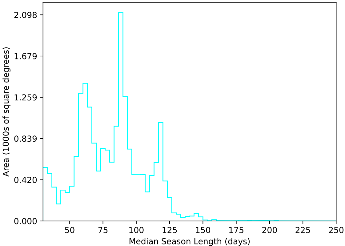
too_10_1v3.4_10yrs All sky u band: Median Season Length
