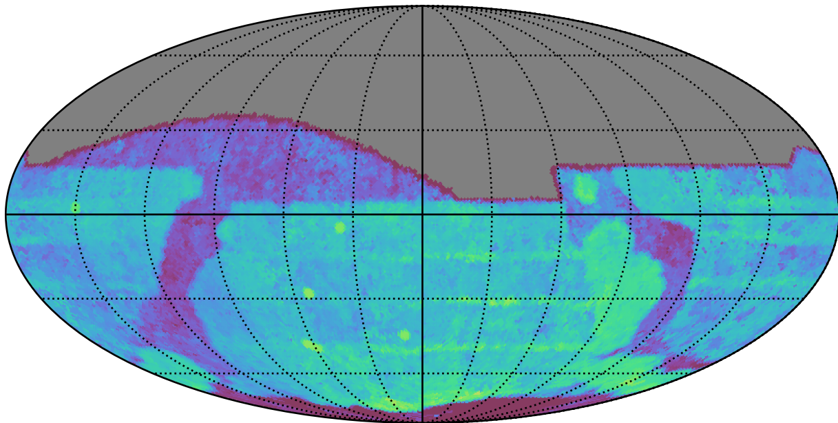
too_10_1v3.4_10yrs All sky r band: Median Season Length
