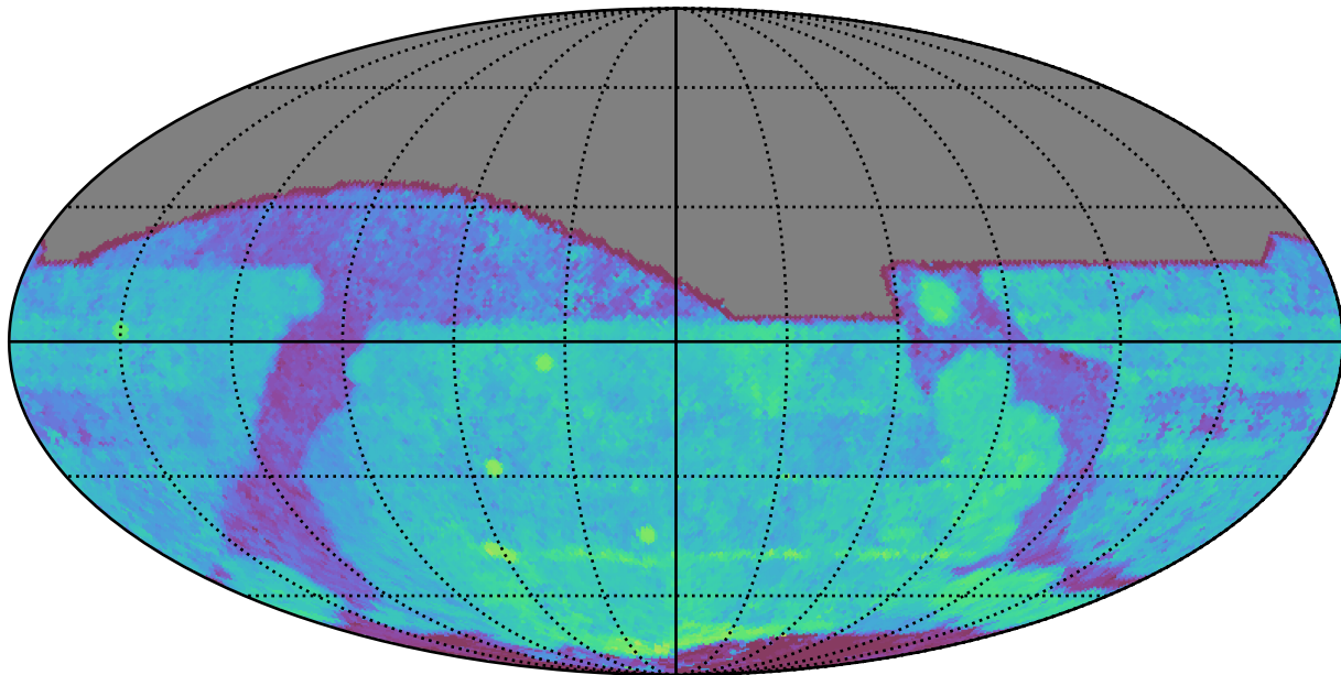
too_10_1v3.4_10yrs All sky i band: Median Season Length
