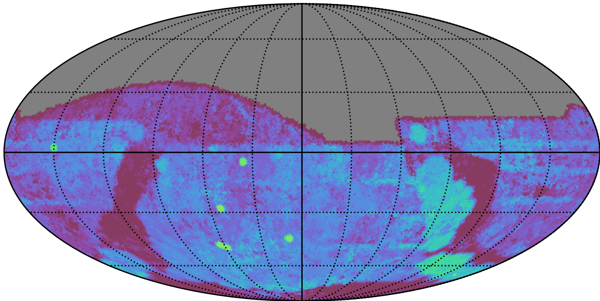
too_10_1v3.4_10yrs All sky g band: Median Season Length
