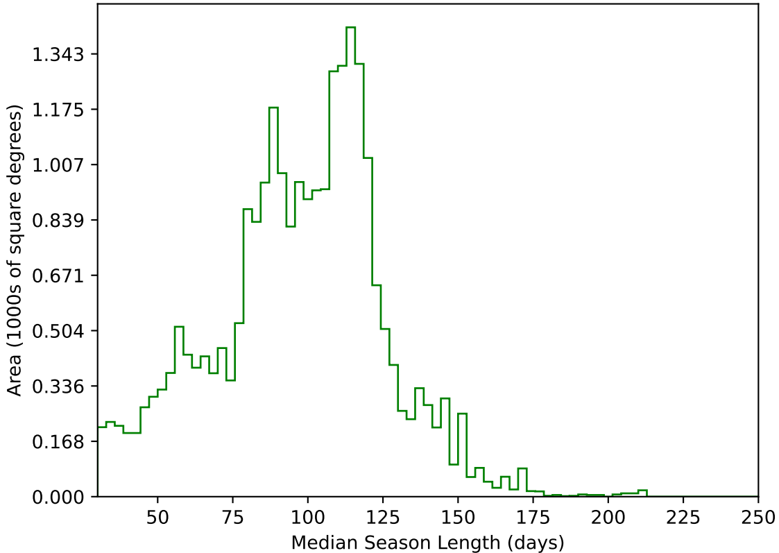
too_10_1v3.4_10yrs All sky g band: Median Season Length
